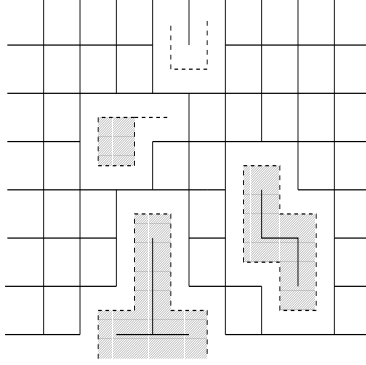
FIGURE 2: A configuration X (full lines) and its A-dual \widehat{X} (dashed lines).
