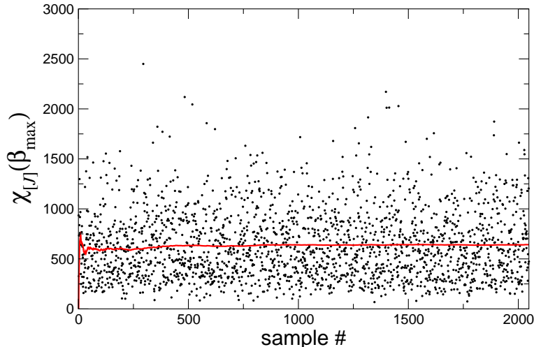
Figure 5: Different values of \chi_{[J]}(\beta_{\max}) (over the samples) of susceptibility at p = 0.56 , L = 96 (the simulation is performed at the temperature of the maximum of the average susceptibility). The running average over the samples is shown by the solid line.
