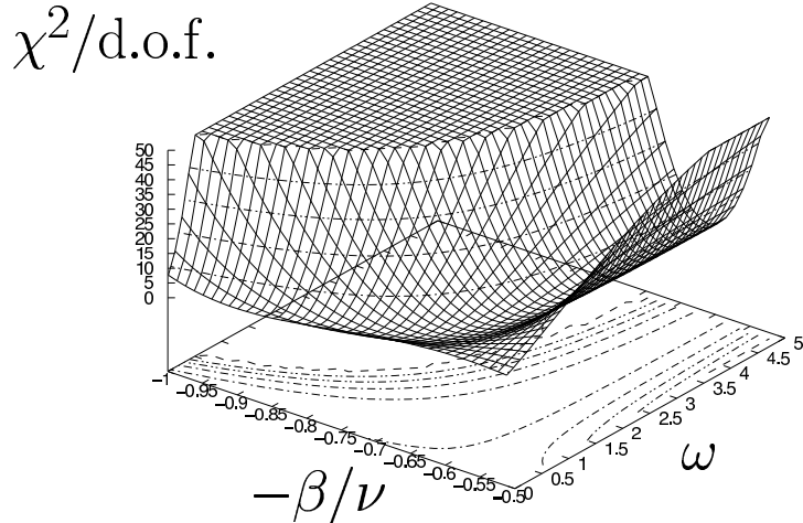
Figure 28: Plot of the \chi^2 deduced from linear fits of \overline{m} (the exponent is thus negative) in the range 25 \leq L \leq 96 for p = 0.56 . In the base plane, the range of variation of the exponents is -1 \leq -\beta/\nu \leq -0.5 and 0 \leq \omega \leq 5 , and the minimum is at \beta/\nu = 0.85 , \omega = 0.135 .
