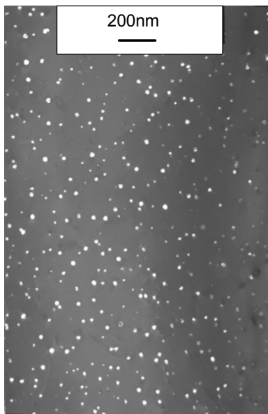
Figure 1: Dark field TEM-micrograph showing the high density of homogeneously distributed \text{Al}_3(\text{Sc,Zr}) -dispersoids after precipitation annealing for 15 hrs at 475°C.
