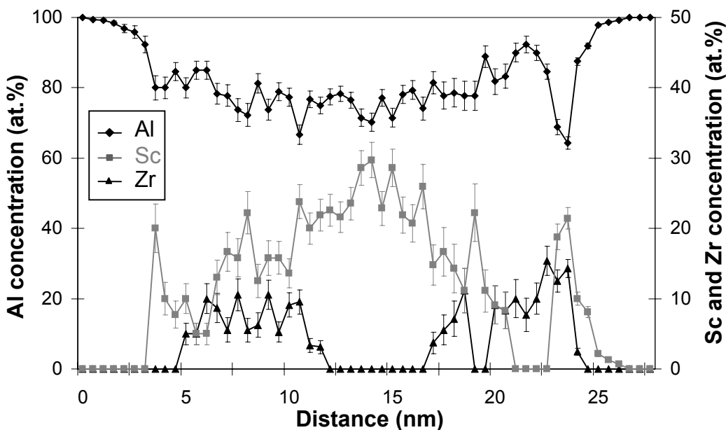
Figure 3: concentration profile through a \text{Al}_3(\text{Sc,Zr}) precipitate
