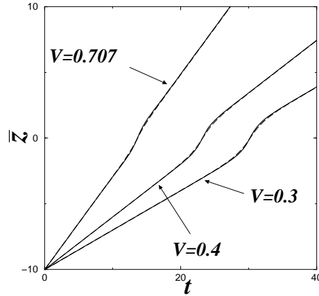
Figure 3: Same as Fig. 2 for solitons incident on an attractive obstacle U(x) = -\delta(x) . The dashed lines corresponding to the effective potential approximation are hardly distinguishable from the solid lines which correspond to the numerical solution of Eqs. (27,28).
