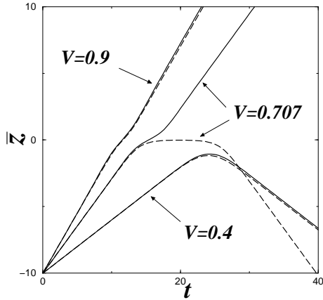
Figure 2: \bar{z}(t) for solitons of initial velocity V , incident on a repulsive obstacle U(x) = \delta(x) . The solid lines correspond to the numerical solution of Eqs. (27,28) and the dashed lines to the effective potential approximation (25).
