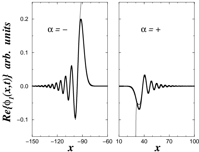
Figure 5: \text{Re}\{\phi_1(x, t)\} as a function of x for \tau = 60 for a soliton of initial velocity V incident on a delta scatterer. The thick line represents the result (57) and the thin line its semiclassical approximation (60). For legibility we have separated the region where \phi_1^- is non zero (around x = -90 ) from the one where \phi_1^+ is non zero (around x = 30 ). Note that in the expected domain of validity of Eq. (60) ( x \gg 30 and x \ll -90 ) one can hardly distinguish the thick line from its semiclassical approximation.
