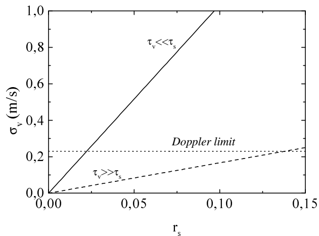
FIG. 6: velocity dispersion \sigma_v for the long (solid line) and short (dashed line) correlation time limit as a function of the relative fluctuation of the intensity r_s = \sigma_s / 2s_0 . In the short correlation time limit \tau_s = 30 \mu\text{s} . The dotted line corresponds to the Doppler limit at low saturation and \Delta = -1 (see text).
