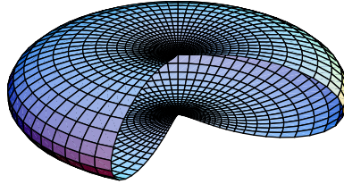
Figure 2: A spherical plot of the electrostatic potential at r = a/2 = \lambda_c/4 (for g = 2 ). For each point on the surface, parametrized by the angles (\theta, \phi) , the value of the potential corresponds to the distance to the origin, r = 0 . Only values of the potential in the directions 0 \leq \phi \leq 3\pi/2 are shown to make the extent of the pinching along the axis more evident.
