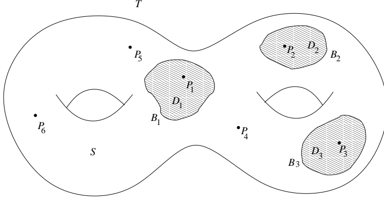
FIGURE 2. The surface T obtained from S by gluing closed discs along its boundary, one for each boundary component.
