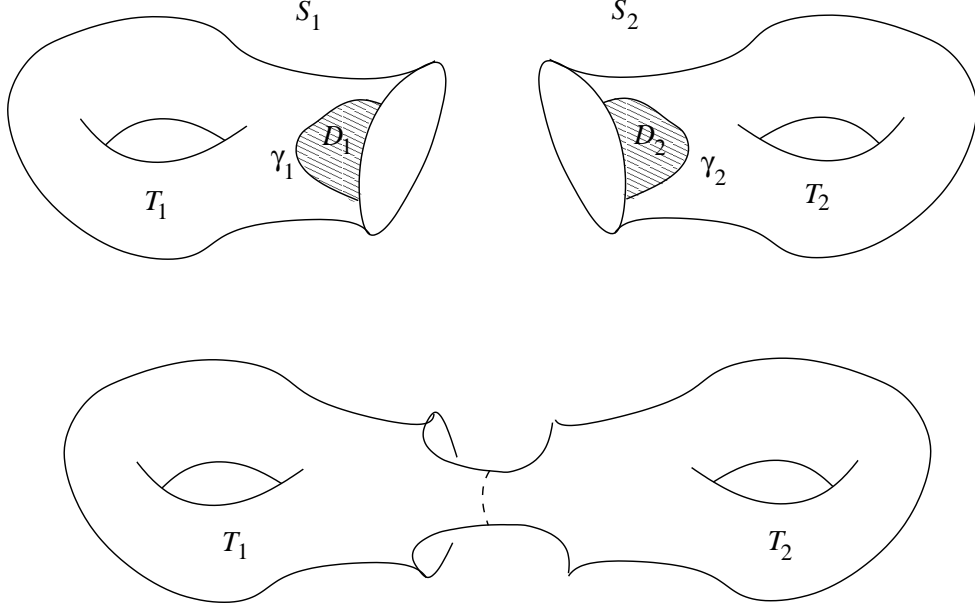
FIGURE 1. The two surfaces T_1 and T_2 are glued together along \gamma_1 and \gamma_2 .
