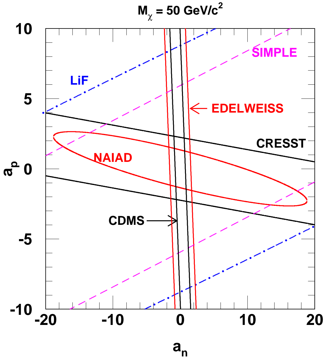
Figure 1: Allowed regions in the (a_n, a_p) plane for M_\chi = 50 \text{ GeV}/c^2 , for the experiments quoted in the text. The region allowed by each experiment is within the corresponding parallel straight lines or ellipse.
