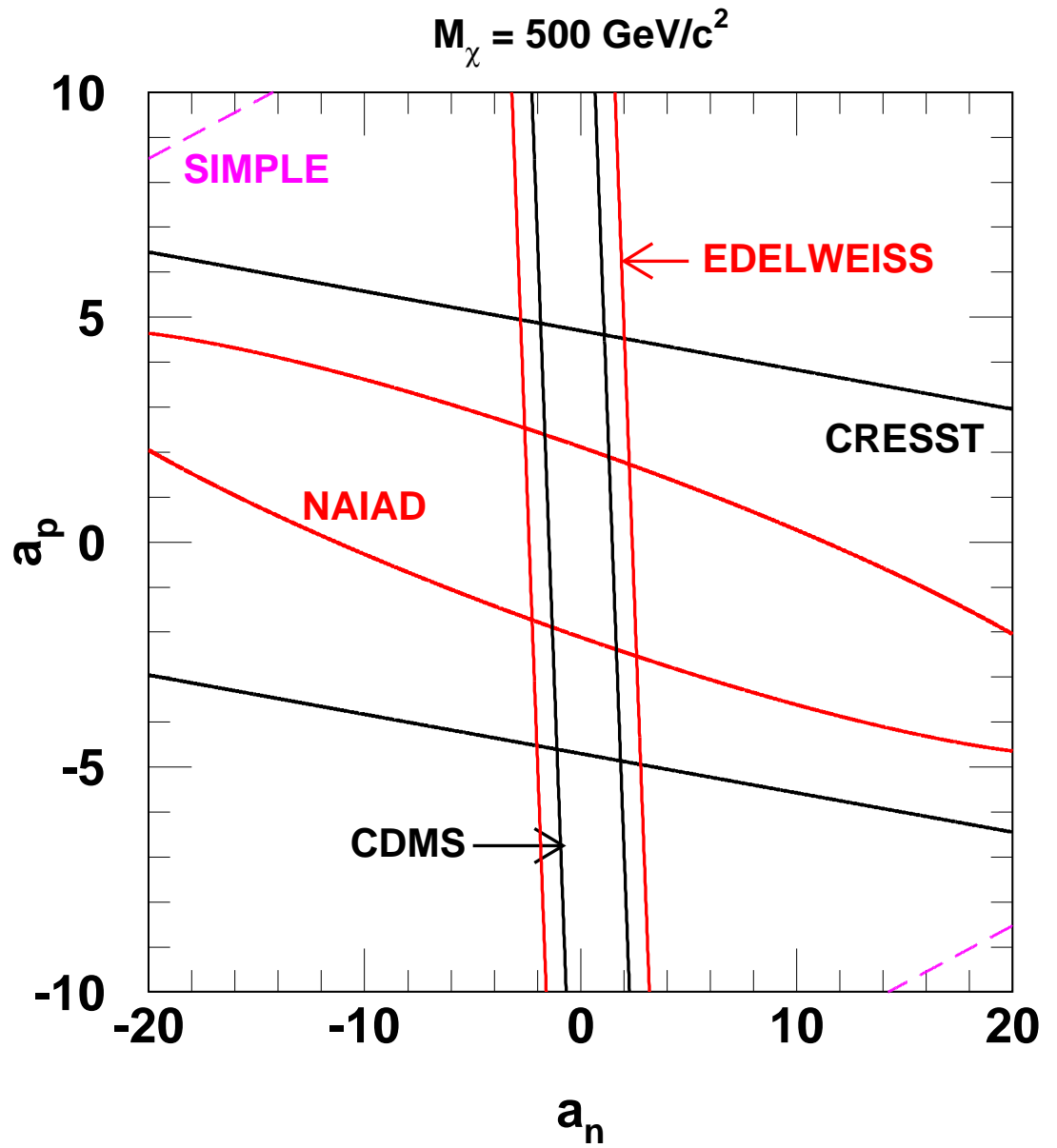
Figure 2: The same as Fig. 1 for M_\chi = 500 \text{ GeV}/c^2 .
