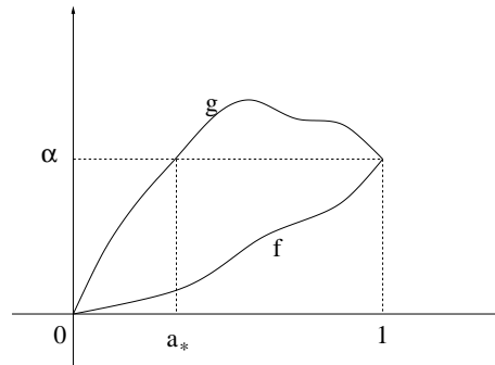
Figure 1: Shape of the functions f and g
