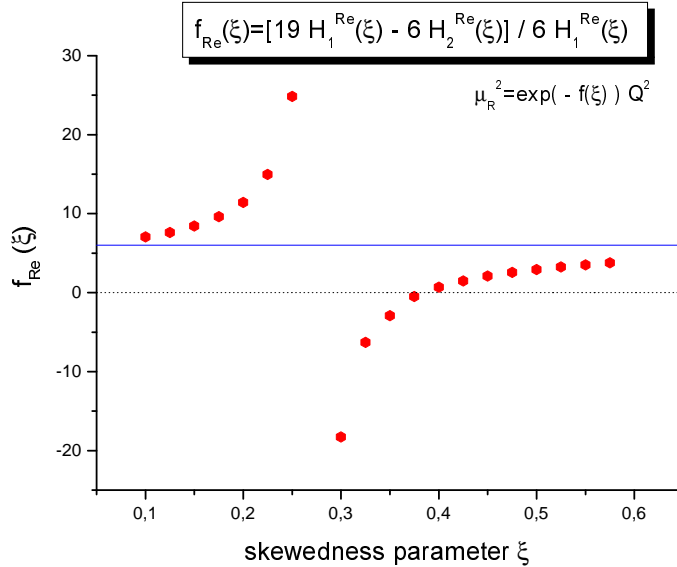
Figure 1: The \rho meson production: the BLM scale for the real part of the amplitude.
