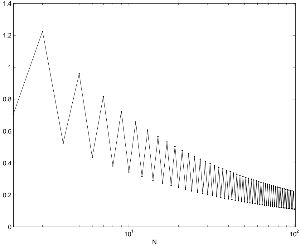
Figure 7: Intertwinement of the lowest positive zeros \lambda_m(N) of the Hermite polynomials H_N and H_{N+1} for small values of N .
