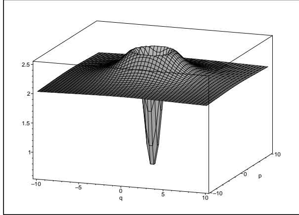
Figure 4: Meanvalue \langle z|H_N|z\rangle of the harmonic oscillator hamiltonian as a function of z = \frac{1}{\sqrt{2}}(q + ip) for N = 5 .
