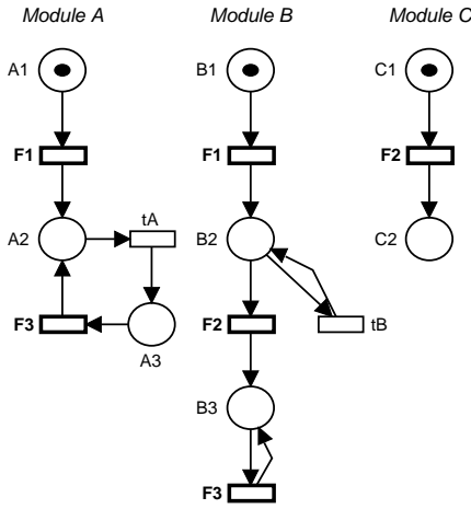
Figure 1. Modular PT-net with modules A, B and C.
