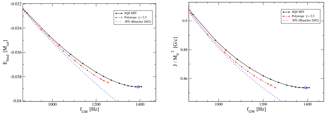
FIG. 5: Binding energy (left panel) and angular momentum (right panel) as a function of gravitational wave frequency along evolutionary sequences of irrotational binaries. The solid line denotes strange quark stars, the dashed one polytropic neutron stars, and the dotted one point-mass binaries in the 3PN approximation [53]. The diamonds correspond to dynamical orbital instability (the ISCO).
