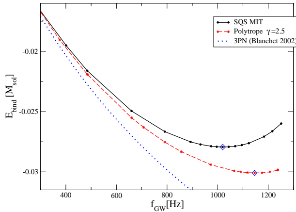
FIG. 4: Binding energy as a function of gravitational wave frequency along evolutionary sequences of corotating binaries. The solid line denotes strange quark stars, the dashed one neutron stars with polytropic EOS, and the dotted one point-mass binaries in the 3PN approximation [53]. The diamonds locate the minimum of the curves, corresponding to the innermost stable circular orbit; configurations to the right of the diamond are secularly unstable.
