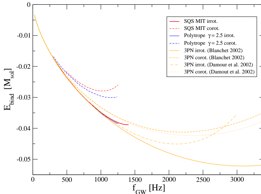
FIG. 8: Binding energy along evolutionary sequences of corotational (dashed lines) and irrotational (solid lines) equal mass binary strange stars and polytropic neutron stars compared with analytical results at the 3rd post-Newtonian order for point-masses by Damour et al. 2000 [54], Damour et al. 2002 [55] and Blanchet 2002 [53]
