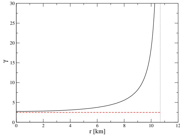
FIG. 3: Adiabatic index \gamma versus the areal radial coordinate r for a static strange star (solid line) and a polytropic neutron star (dashed line). The vertical dotted line corresponds to the stellar surface.
