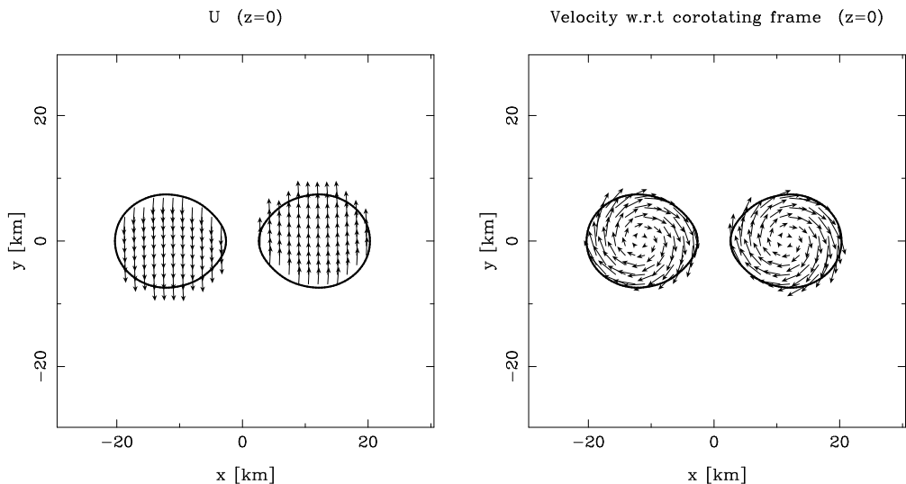
FIG. 6: Internal velocity fields of irrotational strange quark stars binaries at the ISCO. Left panel : velocity \mathbf{U} in the orbital plane with respect to the “inertial” frame (Eulerian observer); right panel : velocity field with respect to the corotating frame. The thick solid lines denote the surface of each star.
