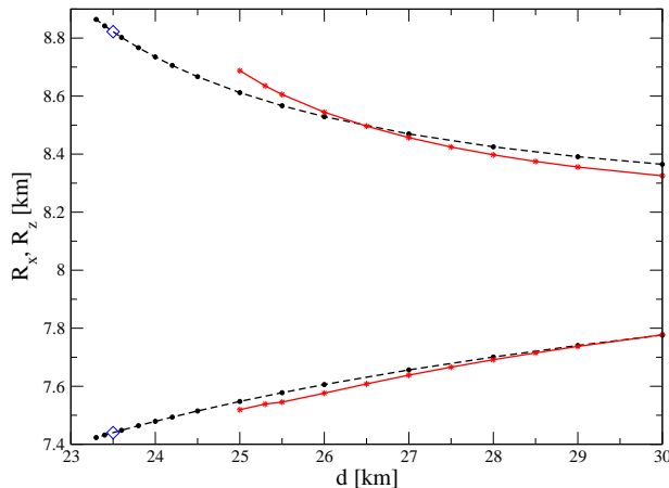
FIG. 7: Coordinate “radius” (half the coordinate size of a star in fixed direction) versus coordinate separation for irrotational quasi-equilibrium sequences of binary strange stars (solid line) and neutron stars (dashed line). Upper lines correspond to equatorial radius R_x (radius along the x axis going through the centers of stars in a binary system) and lower lines are polar radius R_z (radius along the rotation axis).
