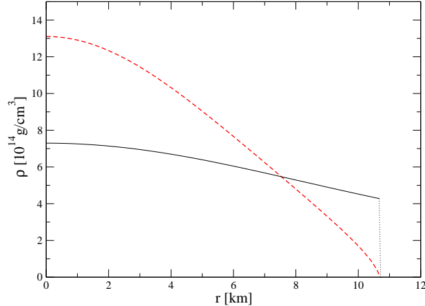
FIG. 2: Density profiles for a static strange quark star (solid line) and a polytropic neutron star (dashed line), having both a gravitational mass of 1.35 M_{\odot} and an areal radius R = 10.677 km (resulting in the compactness parameter M/R = 0.1867 ). The vertical dotted line corresponds to the stellar surface.
