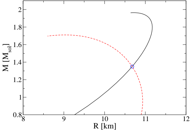
FIG. 1: Gravitational mass M versus areal radius R for sequences of static strange quark stars described by the simplest MIT bag model (solid line) and neutron stars described by polytropic EOS with \gamma = 2.5 and \kappa = 0.0093 m_0 n_{\text{nuc}}^{1.5} (dashed line). The two sequences are crossing at the point M = 1.35 M_\odot and R = 10.677 km (marked by a circle).
