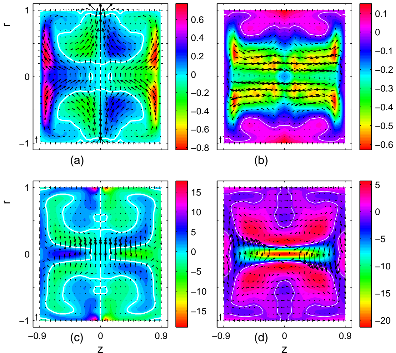
FIG. 15: Meridian sections of \mathbf{B} and \mathbf{j} fields for the neutral mode with w = 0 . \mathbf{B} is divided by the total magnetic energy. Arrows correspond to components lying in the cut plane, and color code to the component transverse to the cut plane. A unit arrow is set into each figure lower left corner. (a): \mathbf{B} field, \theta = 0 . (b) \mathbf{B} field, \theta = \frac{\pi}{2} . (c): \mathbf{j} field, \theta = 0 . (d): \mathbf{j} field, \theta = \frac{\pi}{2} .
