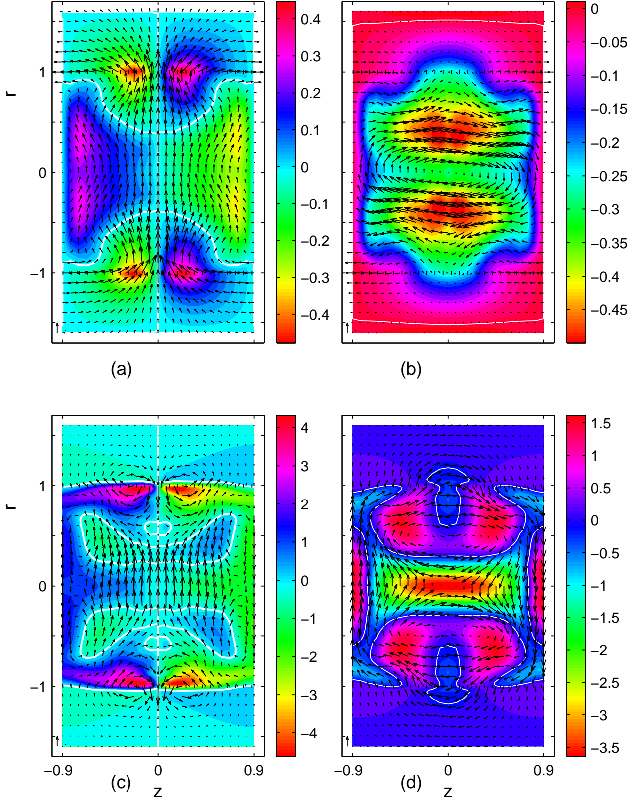
FIG. 18: Meridian sections of \mathbf{B} and \mathbf{j} fields for the neutral mode with w = 0.6 . \mathbf{B} is divided by the total magnetic energy. Arrows correspond to components lying in the cut plane, and color code to the component transverse to the cut plane. A unit arrow is set into each figure lower left corner. (a): \mathbf{B} field, \theta = 0 . (b) \mathbf{B} field, \theta = \frac{\pi}{2} . (c): \mathbf{j} field, \theta = 0 . (d): (c): \mathbf{j} field, \theta = \frac{\pi}{2} .
