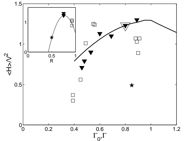
FIG. 20: Mean helicity at a given R_m ( \langle H \rangle / \mathcal{V}^2 ) vs. poloidal over toroidal ratio. The R = 0.75 impeller serie ( \blacktriangledown ) is plotted vs. \Gamma_0 . The large open symbol stands for TM73 at \Gamma_0 and the solid line stands for the same quantity plotted vs. numerical variation of TM73 velocity field ( \Gamma ). We also plot \langle H \rangle / \mathcal{V}^2 vs. \Gamma_0 for the R = 0.5 ( \star ) and R = 0.925 ( \square ) impellers. The inset presents \langle H \rangle / \mathcal{V}^2 vs. impeller radius R for impellers of 0.8 \lesssim \Gamma_0 \lesssim 0.9 .
