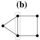
Fig. 7. Smooth bicyclic graphs with one occurrence of triangle.
