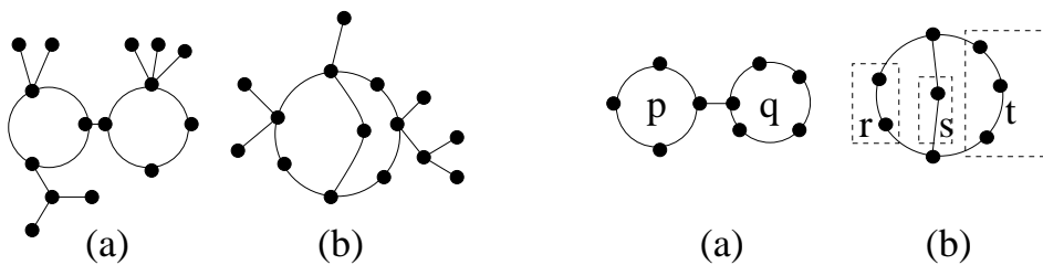
Fig. 4. Examples of bicyclic components. Fig. 5. Smooth bicyclic components.
