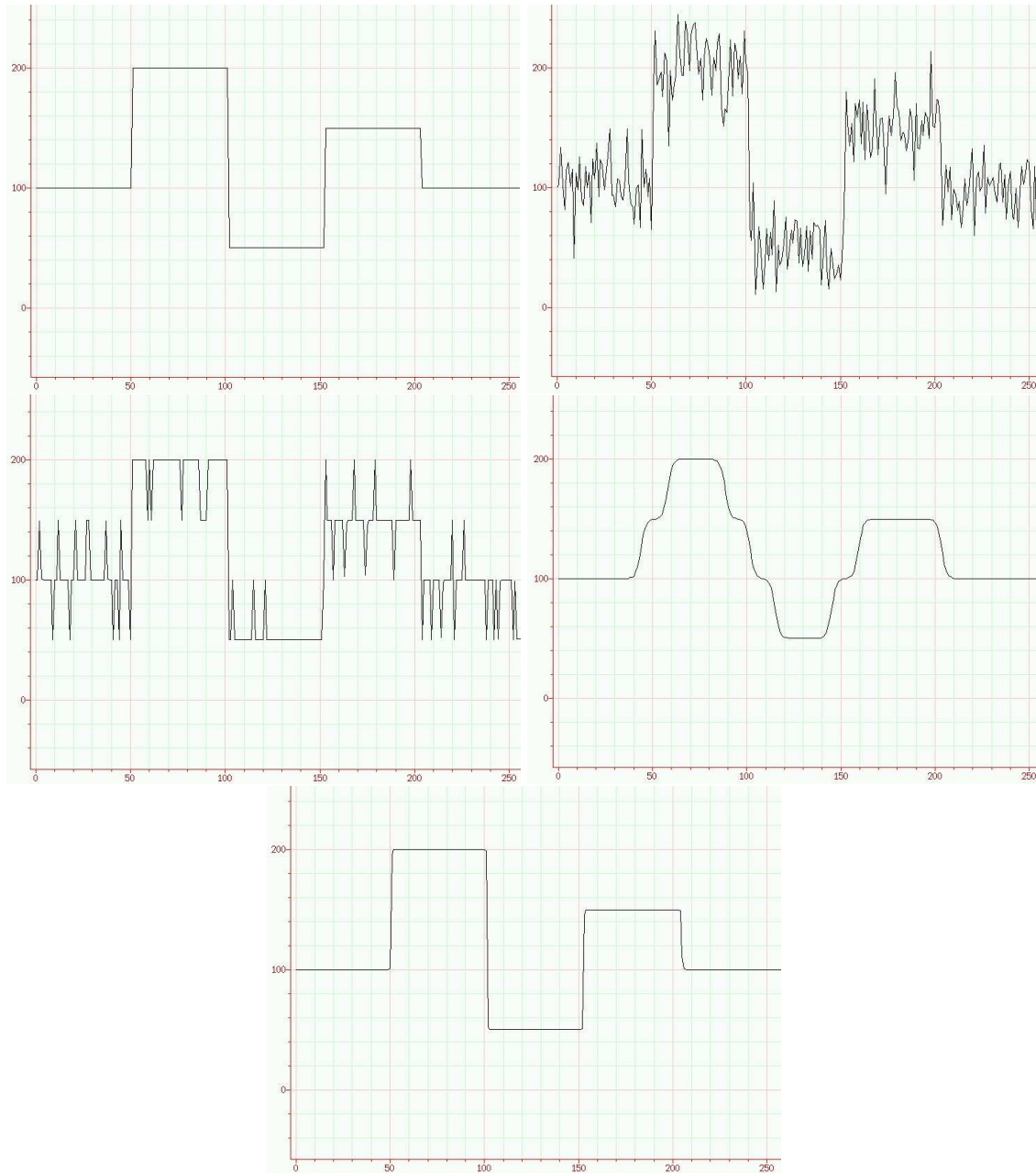
Figure 2: TOP LEFT: (a) piecewise constant signal. TOP RIGHT: (b) Signal (a) with 20% of gaussian noise. MIDDLE LEFT: (c) The quantized version of (b) without denoising operator. MIDDLE RIGHT: (d) Signal (b) quantized by equation du/dt = \Delta u - h(u) . BOTTOM : (e) Signal (b) restored and quantized by our model.
