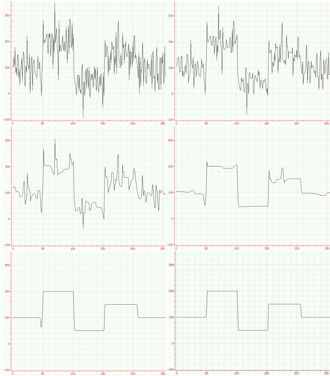
Figure 3: TOP LEFT: (a) Signal (Figure 2-a) with 50% of gaussian noise. TOP RIGHT: (b) t = 10 . MIDDLE LEFT: (c) t = 25 . MIDDLE RIGHT: (d) t = 50 . BOTTOM LEFT: (e) t = 75 . BOTTOM RIGHT: (f) t = 100 .
