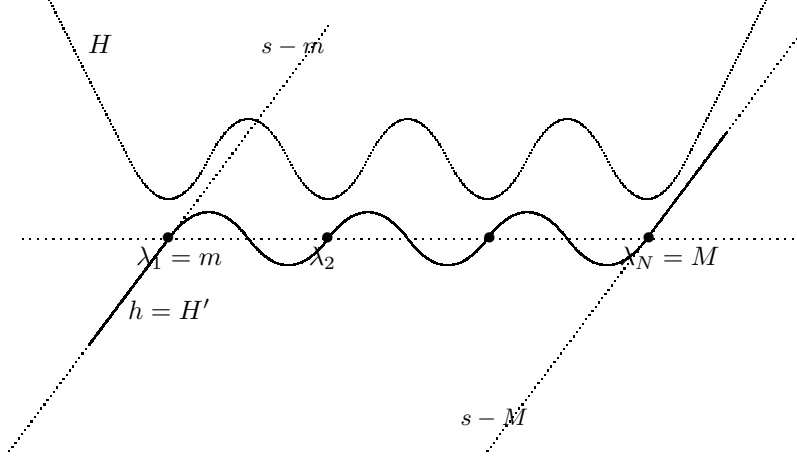
Figure 1: The potential function H and its derivative.
