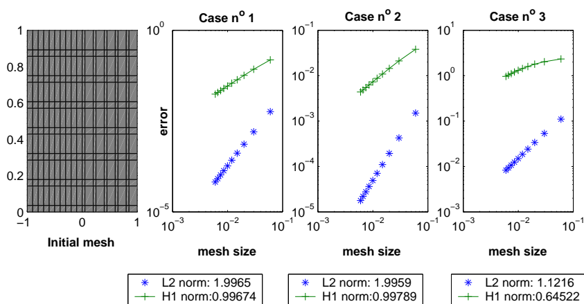
Figure 6: Convergence order of the FVD scheme for a regular solution on a regular mesh
