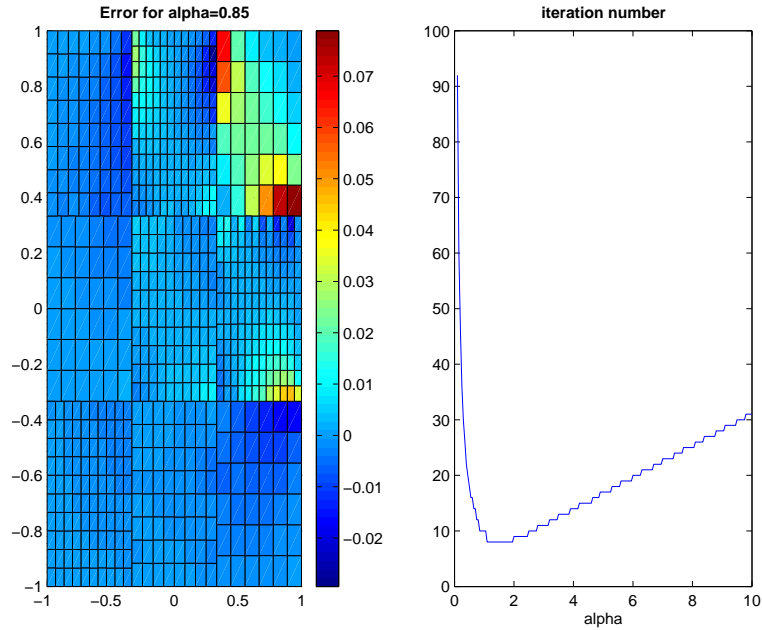
Figure 10: Error estimate between the Schwarz algorithm and the FVD scheme for Case n°3, \varepsilon = 1 .
