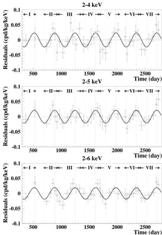
Fig. 4. Annual modulation amplitude reported by the DAMA experiment using a \sim 10^5\text{ kg} \times \text{day} data sample, recorded over a period of seven years. The statistical significance of the detected modulation is \sim 6.2 standard deviations (from Bernabei et al. Ref. [52])
