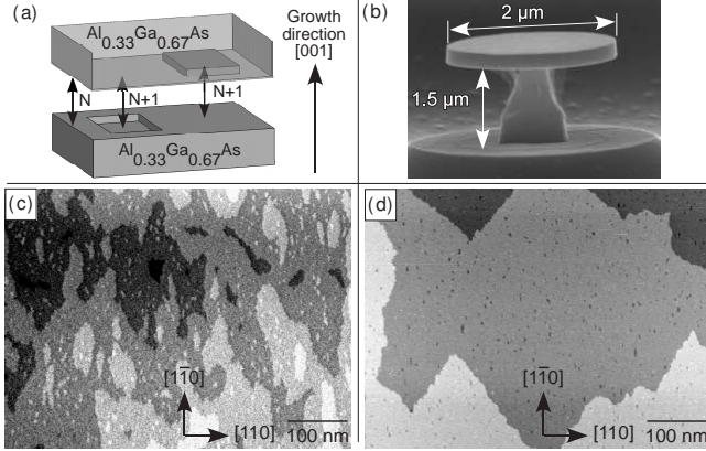
FIG. 1: (a) Schematic of a monolayer fluctuation QD. (b) Scanning electron microscopy sideview of a 2 \mu m diameter microdisk. (c) 800nm * 600nm Scanning tunnelling microscopy (STM) image of the surface after the deposition of the first 50 nm Al_{0.33}Ga_{0.67}As barrier and after the growth interruption; the color changes correspond to one (AlGa)As monolayer changes in height (d), STM image of the surface after growth of the 13 monolayer GaAs QW and after the growth interruption.
