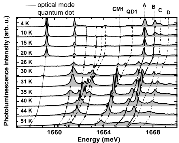
FIG. 2: Photoluminescence spectra (vertically shifted for clarity) on a single microdisk at various temperatures from 4 K to 51 K. The dotted (resp. dashed) lines are guides to the eye to follow the emission energy of the optical modes (resp. quantum dot excitons). Solid lines follow spectral shifts different both from a quantum dot and an optical mode spectral shift.
