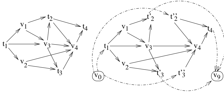
FIGURE 2. A graph G and its associated graph \widehat{G}
