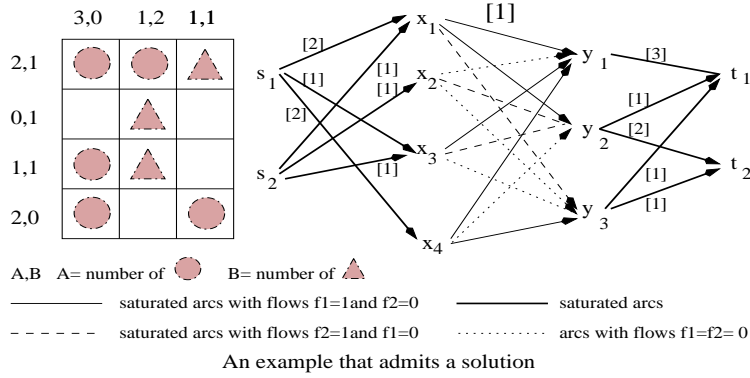
FIGURE 4. Matrix reconstruction and bipartite multiflow.
