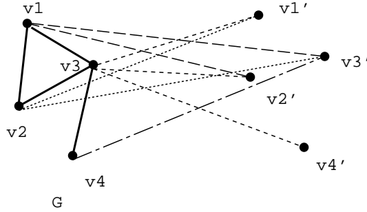
FIGURE 1. IMFP with demands and INDEPENDENT SET problems
