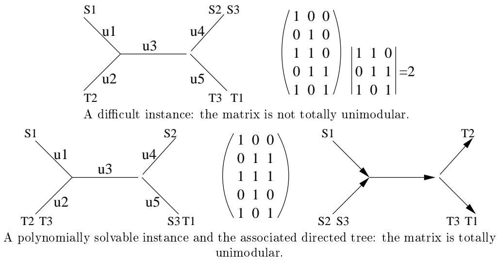
FIGURE 3. Easy and difficult instances in undirected trees.
