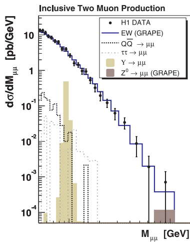
Figure 3. Differential muon pair production cross-section as a function of di-muon mass, from the H1 analysis.
