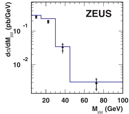
Figure 2. Differential muon pair production cross-section as a function of the invariant mass of the muon pair M_{\mu\mu} , measured by the ZEUS Collaboration.
