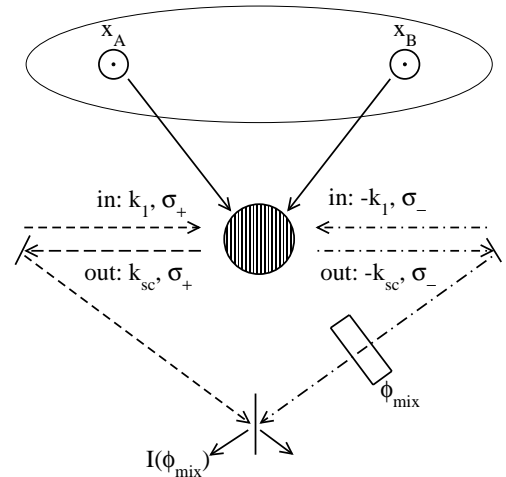
FIG. 2: Second proposed set-up: atoms are extracted from the cloud at \mathbf{x}_{A,B} and create a matter-wave grating when the wave-packets overlap at \mathbf{X} ; one detects this grating by shining a pair of counter-propagating, \sigma_\pm polarized laser beams on the overlap region and by beating the two resulting backscattered light beams on a beam splitter: as function of the mixing phase \phi_{\text{mix}} , the beating intensity I(\phi_{\text{mix}}) averaged over many realizations presents fringes revealing the pair long range order. Dashed (dot dashed) lines: \sigma_+ ( \sigma_- ) polarization.
