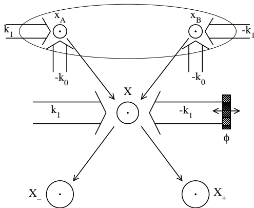
FIG. 1: First proposed set-up: atoms are extracted by a Bragg process from the gas at points \mathbf{x}_{A,B} , using pairs of laser beams of wavevectors -\mathbf{k}_0, \mathbf{k}_1 and -\mathbf{k}_0, -\mathbf{k}_1 respectively; at their overlap position \mathbf{X} , the two atomic wave-packets are coherently mixed by a laser standing wave acting as a 50-50 beam-splitter with adjustable phase shift \phi ; the number of atoms in each wave-packet is measured at the final positions \mathbf{X}_\pm .
