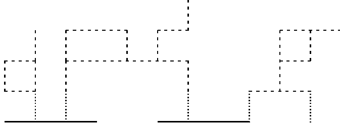
FIGURE 2 : A hydra, in two dimensions (a dimension not considered in this paper), with 2 feet (components of full lines), 5 necks (dotted lines), and 3 heads (components of dashed lines).
