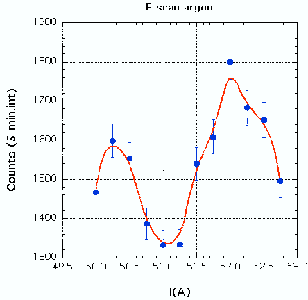
FIGURE 3. He-like argon M1 line intensity dependency versus the superconducting coils current. 55 A corresponds to a magnetic field value of 2.35 kG at the center of the ECRIT.
