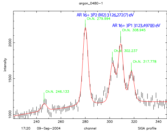
FIGURE 4. He-like and Li-like argon spectrum using quartz [10-1] crystal. HF power injected P = 400 W, argon partial pressure p_{Ar} = 5 \cdot 10^{-9} mbar, total pressure p_{tot} = 5 \cdot 10^{-7} mbar
