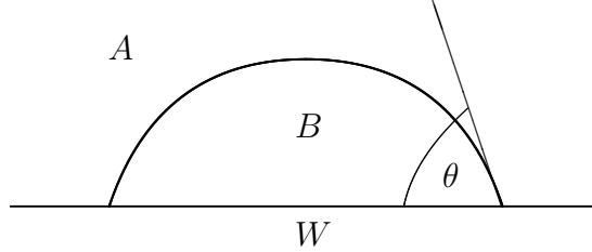
Fig. 1: Young's contact angle
