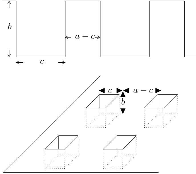
Fig. 4: The substrate surface W in dimensions 1 and 2.
