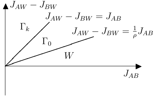
Fig. 5: The diagram of ground states.
