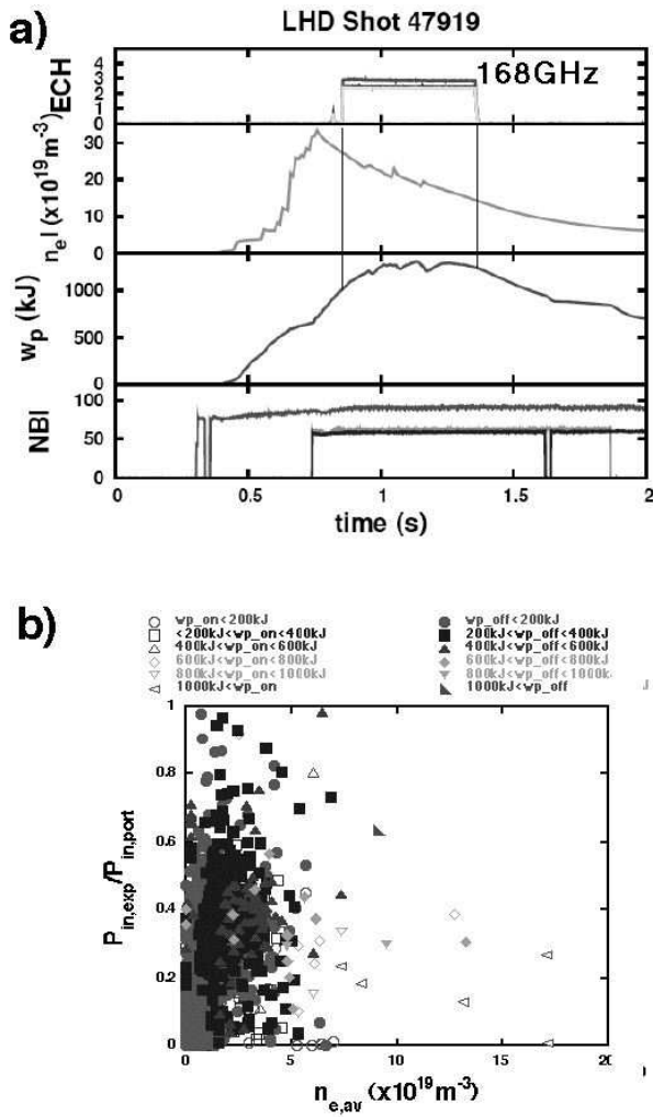
Figure 5. a)Effect of 168 GHz second harmonic heating at high density plasma where the highest stored energy of 1.3MJ is recorded. b)Dependence of the heating efficiency of 168 GHz injection on target plasma density
