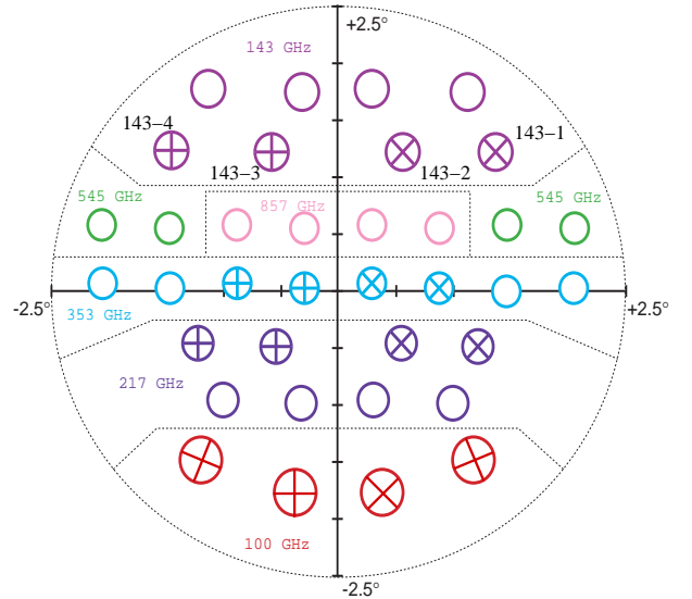
(a) Fig. 2. Planck focal plane unit (FPU) with polarization sensitive bolometers as seen from the sky. Complementary pairs of PSB detectors are arranged in two horns following each other while scanning the sky so that four detectors are in an optimized configuration for polarization measurement.
