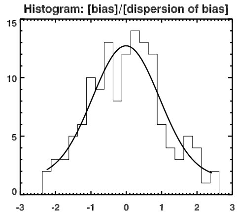
Fig. 5. Histogram of the biases divided by the statistical dispersion for all multipole bins shown on figure 4. As expected, the histogram is well fitted by a Gaussian of unit variance, showing that the dispersion on 450 simulations gives a good estimate of the errors.
