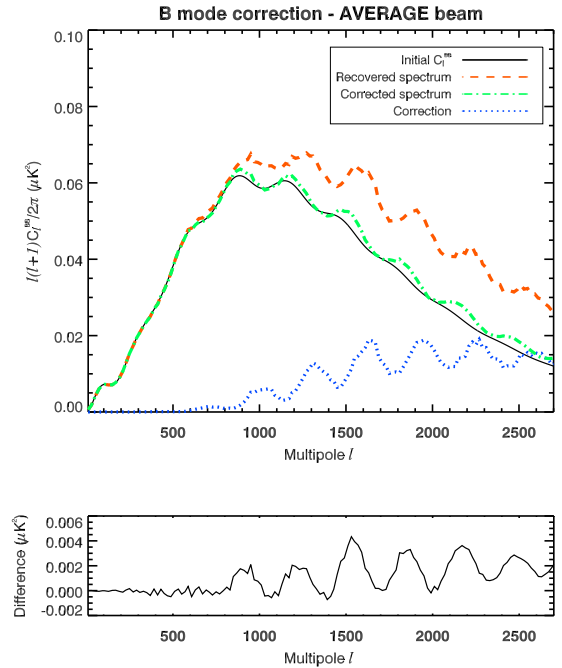
Fig. 11. Recovered B mode power spectrum before (red, dashed line) and after (green, dot-and-dashed line) correction. The power spectrum is corrected by subtracting the estimated leakage (blue dotted line) using beams averaged within one horn (0.5% error, see text). Bottom: Difference between corrected and initial power spectra.
