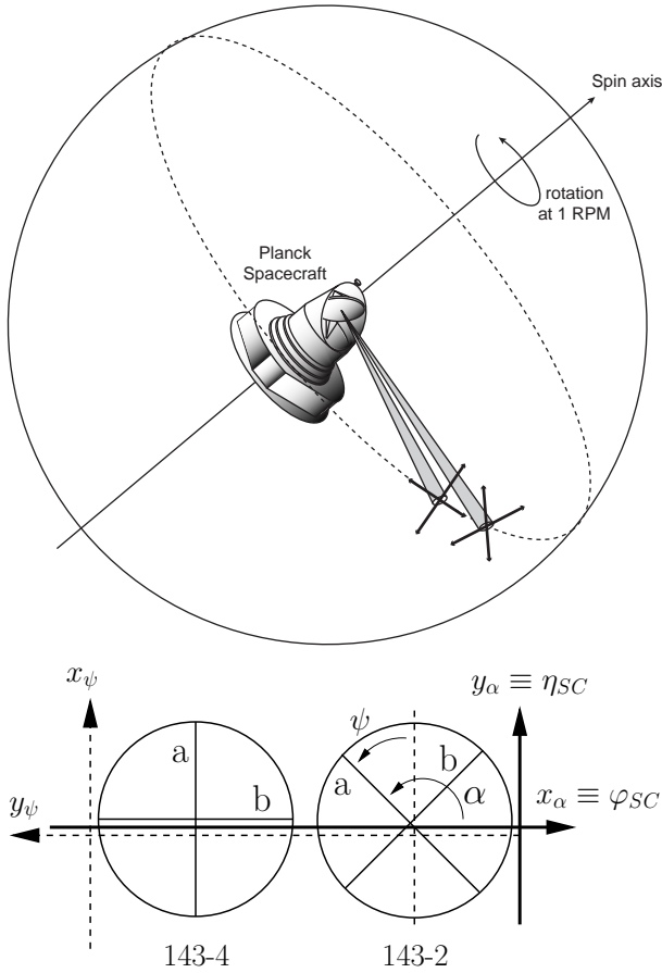
Fig. 1. (a) The scanning of the polarized detectors provides the measurements of intensity of the CMB field components along four directions at each point on the scan path. (b) Definition of axis specifying the Stokes parameters reference frame as seen from the sky. The detector pair on the left ( e.g. 143-4) measures the Q Stokes parameter, while the pair on the right ( e.g. 143-2) measures U when Q and U are defined with respect to the (x_\alpha, y_\alpha) frame (see Appendix A for further detail on reference axis).
