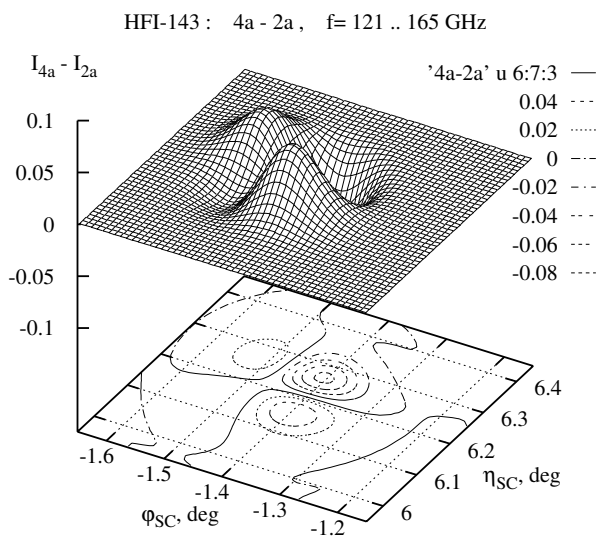
Fig. A.1. Relative difference of power patterns (a) \tilde{I}_{4a} - \tilde{I}_{4b} of two orthogonal channels of the same beam HFI-143-4 ( \psi = 0^\circ and \psi = 90^\circ , respectively) and (b) \tilde{I}_{4a} - \tilde{I}_{2a} of the channels HFI-143-4a and HFI-143-2a ( \psi = 0^\circ and \psi = 45^\circ , respectively) when superimposed by spinning the telescope about the geometrical spin axis.
