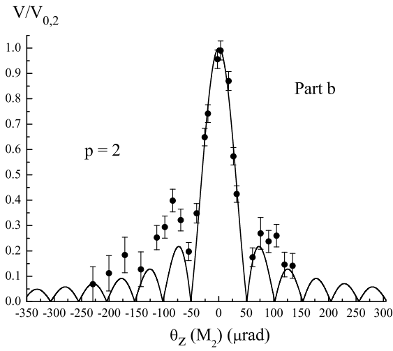
FIG. 5: Fringe visibility measured as a function of the angle \theta_z measuring rotation around the \mathbf{z} -axis of mirror M_2 . The experiment has been done with the diffraction orders p = 1 (part a) and p = 2 (part b). The points are experimental and the curves are the best fits using equation (12). The agreement is excellent in the central region, where the visibility decreases twice as fast as when using p = 2 than when using p = 1 , in agreement with equation (12).
