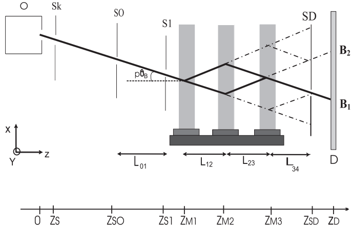
FIG. 1: Schematic drawing of our Mach-Zehnder interferometer (top view). The x, y, z axis are represented and we give the distance z of each element to the nozzle. O : lithium oven; Sk : diameter skimmer at z_s = 20 mm ; S_0 : first collimating slit at z_{S_0} = 485 mm; S_1 : second collimating slit at z_{S_1} = 1265 mm; M_i, i = 1 - 3 : mirrors for the laser standing waves at z_{M_1} = 1415 mm, z_{M_2} = 2020 mm and z_{M_3} = 2625 mm; B_1 and B_2 : complementary exit beams; S_D : detector slit with a tunable width at z_{S_D} = 3025 mm ; D : 760 \mu\text{m} wide rhenium hot wire of the Langmuir-Taylor detector at z_D = 3375 mm. We have also represented the main stray atomic beams produced by diffraction on the three gratings, assuming that only two diffraction orders, 0 and p are produced, as in the ideal Bragg regime.
