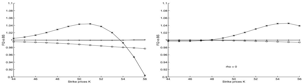
Figure 8: Is pricing a Heston Call using functional quantization (with Romberg log-extrapolation) more performing than using Black-Scholes formula? ---*---: (BS price)/(Heston price), ---o---: (FQ 9984 Price)/(Heston price), ---+---: (FQ Romberg log-extrapolated price)/(Heston price).
