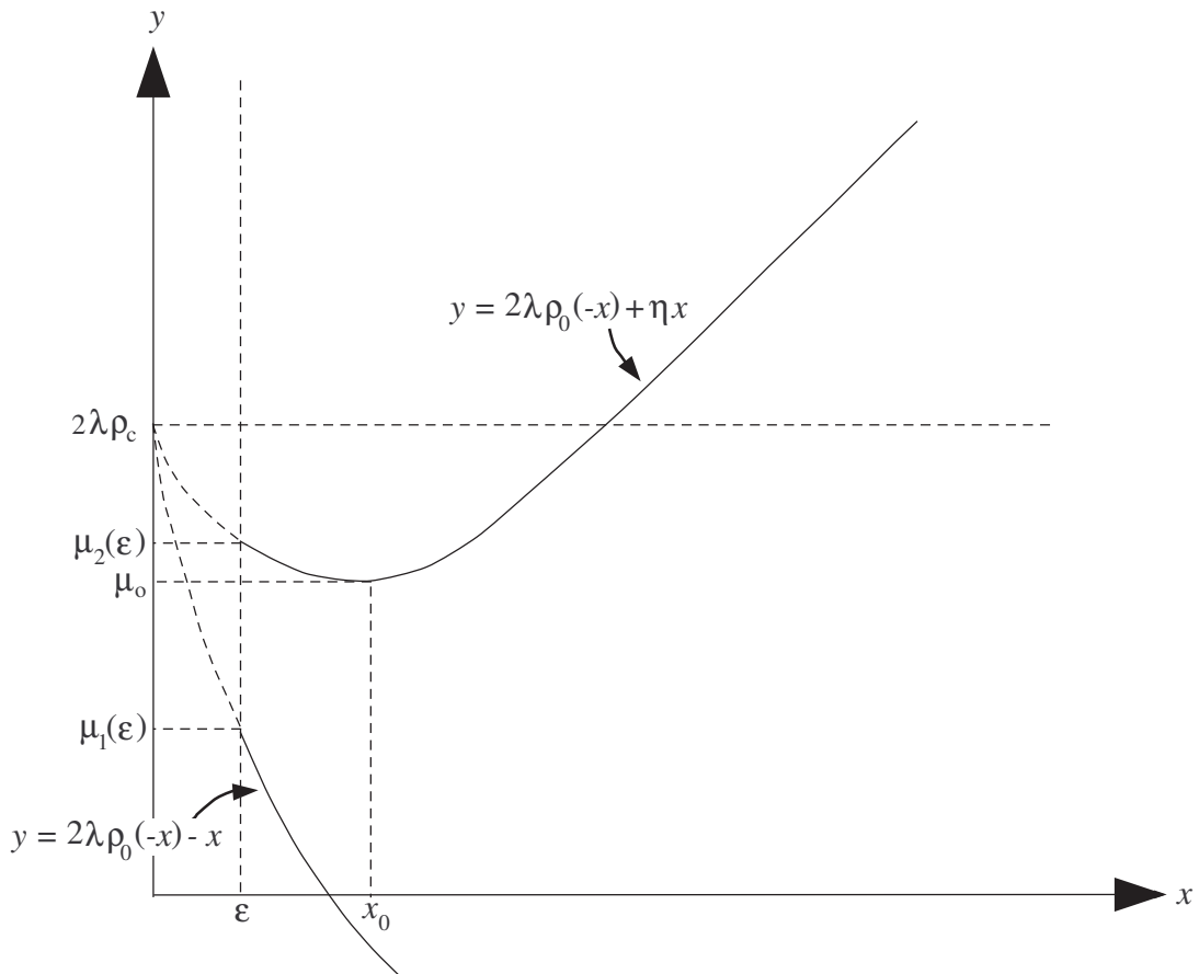
Figure 1: Solution of the density equation
