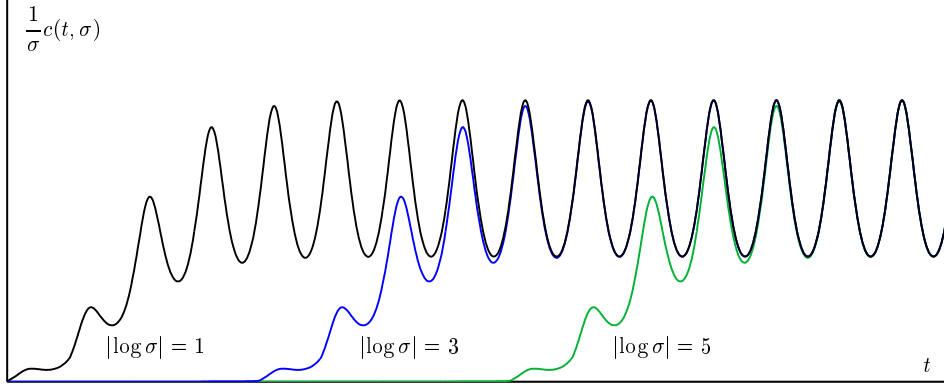
FIGURE 3. The prefactor c(t, \sigma) of the first-passage density as function of time, for different values of \sigma . After a transient regime of duration 2|\log \sigma|/\lambda , the density approaches a periodic function of time. Only for times exponentially large in 1/\sigma^2 will the density show a visible decay.
