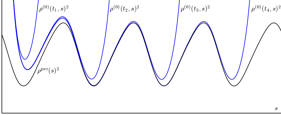
FIGURE 7. The functions \rho^{\text{per}}(s)^2 and \rho^{(0)}(t_i, s)^2 for four different final times t_1 < t_2 < t_3 < t_4 .
