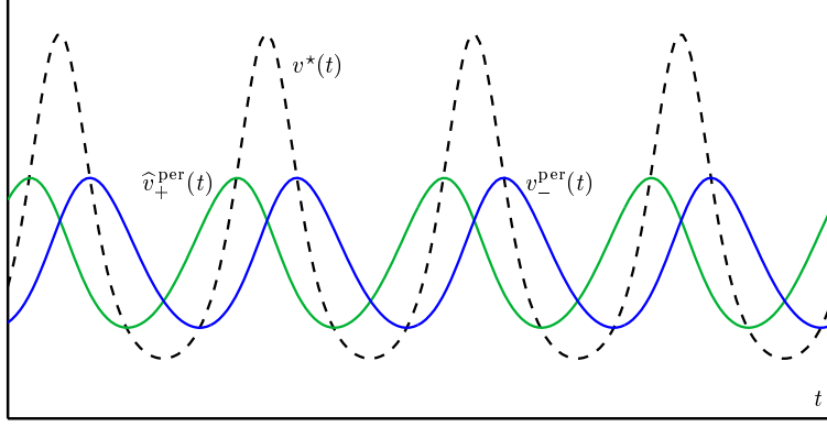
FIGURE 2. The periodic functions v^*(t) , v_-^{\text{per}}(t) and \widehat{v}_+^{\text{per}}(t) .
