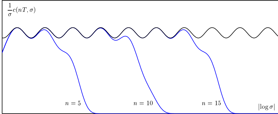
FIGURE 4. The prefactor of the first-passage density as function of |\log \sigma| , for three different values of t = nT . The prefactor is close to a periodic function of |\log \sigma| for 2|\log \sigma| \leq \alpha(nT) = \lambda nT , and decreases exponentially, with an exponent proportional to -const e^{-\alpha(nT)} / \sigma^2 , for 2|\log \sigma| > \alpha(nT) = \lambda nT .
