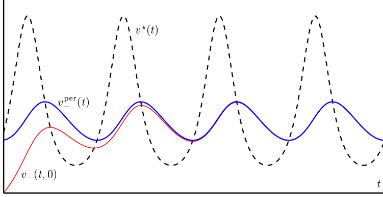
FIGURE 6. The functions v_-(t, 0) and v_-^{\text{per}}(t) .
