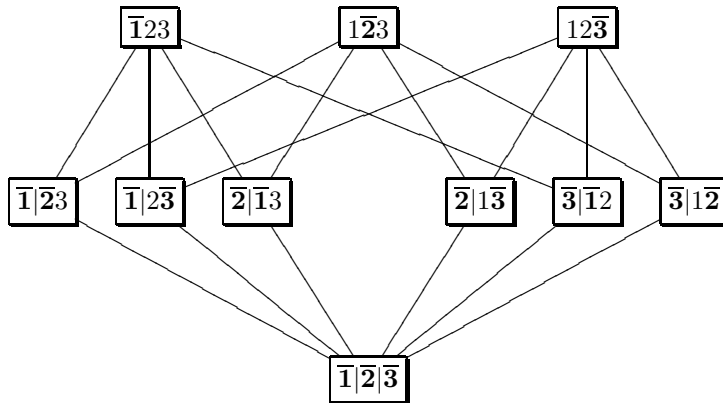
Figure 1: The poset \Pi_3^A
