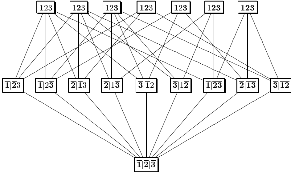
Figure 3: The poset \text{MII}_3^A
