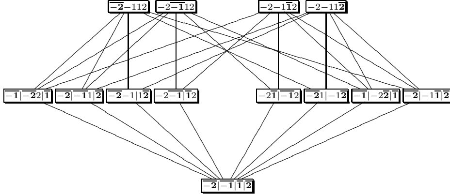
Figure 2: The poset \Pi_2^B
