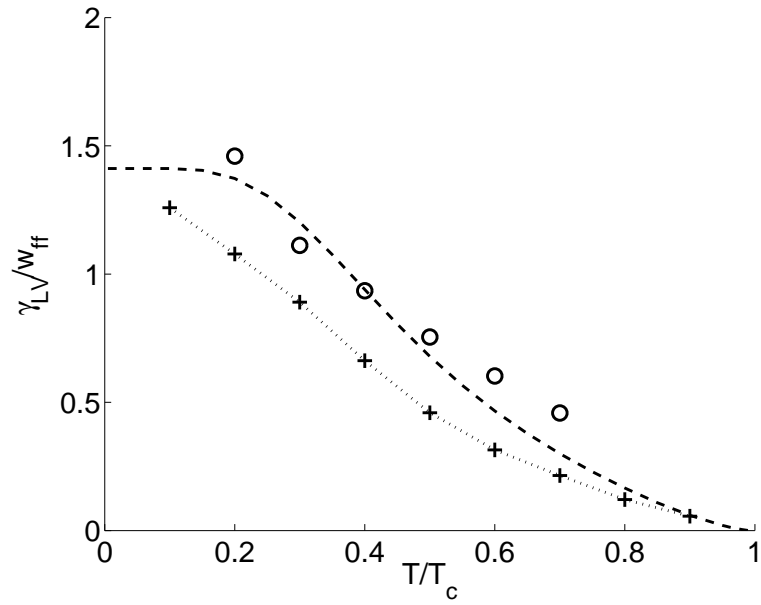
FIG. 4 – Monte Carlo estimate of liquid-vapor surface tension as a function of T/T_c . Dotted line with crosses : mechanical estimate (implemented in the Monte Carlo sampling) in the [110] direction. Circles : estimate from the free energy calculation of a liquid bubble (see text for details). Dashed line : mean field calculation for the [110] interface.
