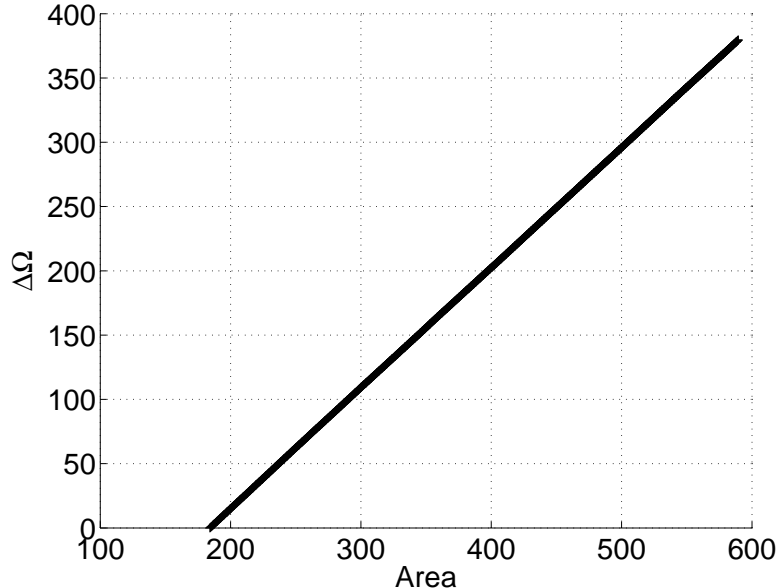
FIG. 5 – Umbrella sampling estimate of the liquid vapor \gamma_{LV} . The measured grand potential is plotted as a function of the liquid-vapor area. Numerical parameters are T/T_c = 0.4 and \mu/w_{ff} = -4.0 (corresponding to the liquid-vapor coexistence). The stiffness \kappa of the biasing potential is \kappa = 0.01 and the total system size is 2 \times 10^3 sites.
