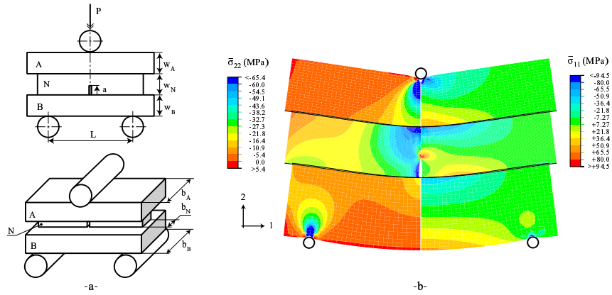
Figure 1. a-Schematic and main dimensions of a sandwiched-beam geometry. b-Average stress fields obtained by FE simulations when f = 0.3 , F = 2000 N, \alpha = 0.4 for a magnified deformed shape ( b_A = 9 mm, b_B = 9 mm, b_N = 3 mm, w_A = 5.5 mm, w_B = 7 mm, w_N = 5 mm, E_A = E_B = 210 GPa, E_N = 410 GPa).
