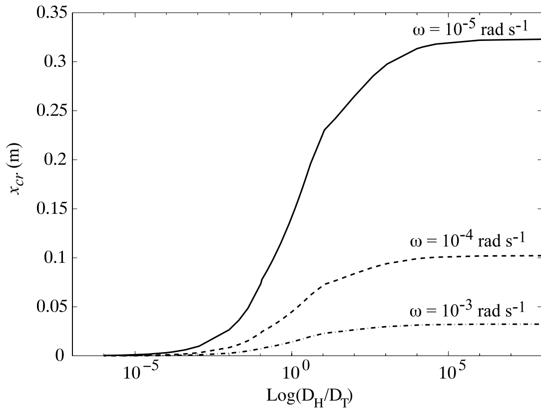
Figure 5. Influence of the frequency \omega and the diffusivity ratio on the abscissa x_{cr} (approximate solutions for D_T = 10^{-7} \text{ m}^2 \text{ s}^{-1} )
