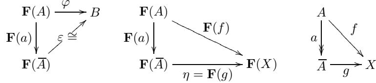
FIGURE 3.1. Projectability of the functor \mathbf{F} .
