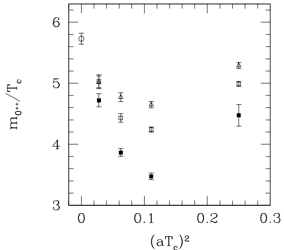
Figure 2. m_{0^{++}}/T_c for \beta_a = 0 (filled squares) \beta_a = -2 (open squares) and \beta_a = -4 (triangles) as function of (aT_c)^2 . The circle gives the continuum results extracted from the literature.
