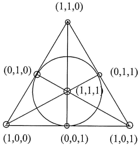
Figure 1: The Fano plane.
