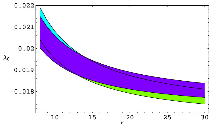
Figure 4: The dependence of \lambda_0 on r . The darker shaded region indicates the range of values Eq. (3.15) for \lambda_0 determined by using V_{ud} from superallowed nuclear beta decay, while the lighter shaded region shows the corresponding range Eq. (3.16) determined by using the PDG values for V_{us} . See text for details.
