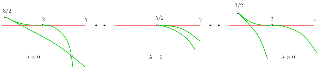
Figure 2: Envelope perestroika of singularity S_{1,1} .
