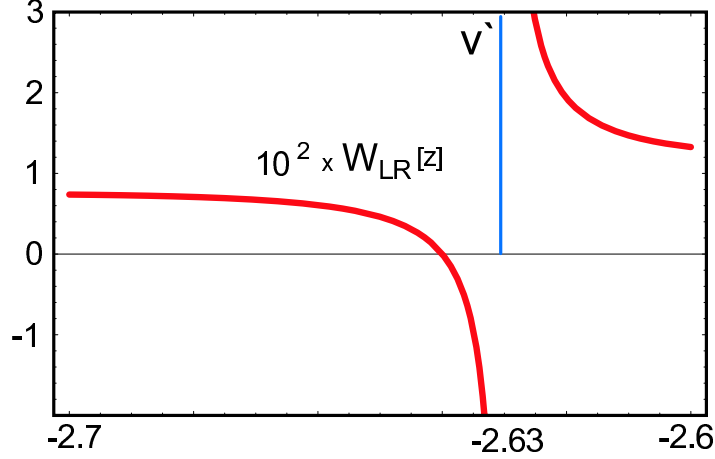
Fig. 2c The predicted shape of the function W_{LR}[z] in the V' region.
