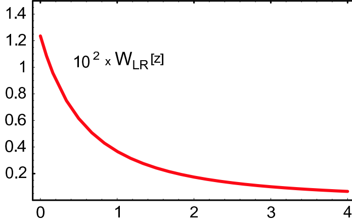
Fig. 2a The predicted shape of the function W_{LR}[z] in Eq. (3.1) in the euclidean.
