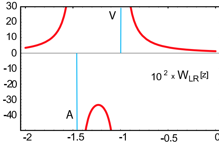
Fig. 2b The predicted shape of the function W_{LR}[z] in Eq. (3.1) in the Minkowski region -2 \leq z \leq 0 . The vertical lines are the delta functions contributing to the imaginary part, the continuous solid lines, are the shape of \text{Re}W_{LR}[z] in that region.
