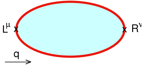
Fig. 1 Feynman diagram representing the \Pi_{LR} correlation function in Eq. (1.2) in the large- N_c limit. The solid lines are light quarks propagating in a gluonic background of large- N_c planar diagrams.
