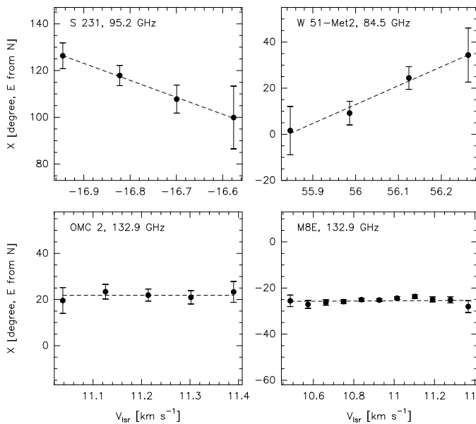
Fig. 9. Polarization angle profiles of Class I \text{CH}_3\text{OH} masers. The ordinates are all at the same scale, to better compare the end-to-end difference of polarization angles. The flat profiles (bottom row) are clearly distinguished from those with a slope (top row).
