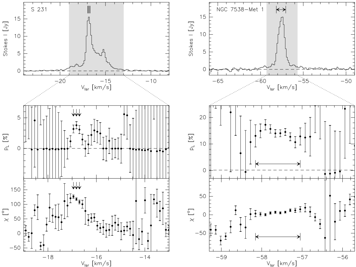
Fig. 3. Class I methanol masers at 95 GHz.
