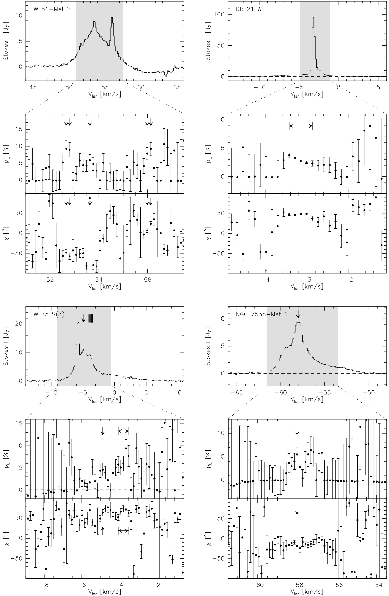
Fig. 2. Class I methanol masers at 84 GHz. For each source, Stokes I (top), the fractional linear polarization p_L (center), and the polarization angle \chi (E from N, bottom) are shown, with spectral baselines subtracted. Vertical bars or arrows and horizontal arrows mark the velocities or velocity ranges, respectively, with p_L > 3\sigma_{\text{rms}} . The grey-shaded areas in the Stokes I spectra indicate the velocity range for p_L and \chi .
