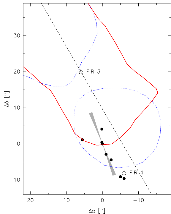
Fig. 7. Schematic representation of methanol masers in OMC-2. Black dots: 44 GHz masers of Kogan & Slysh (1998). Contours: extent of the overlapping outflow system (in CO(1-0), from Williams et al., 2003). The dashed straight line is the outflow axis. Dotted contours: blue shifted lobes. Solid contour: red shifted lobe. The polarization angle of our 133 GHz measurement and its error are indicated by the shadowed line (whose length is the beamwidth, FWHM). The positions of the FIR sources are from Chini et al. (1997).
