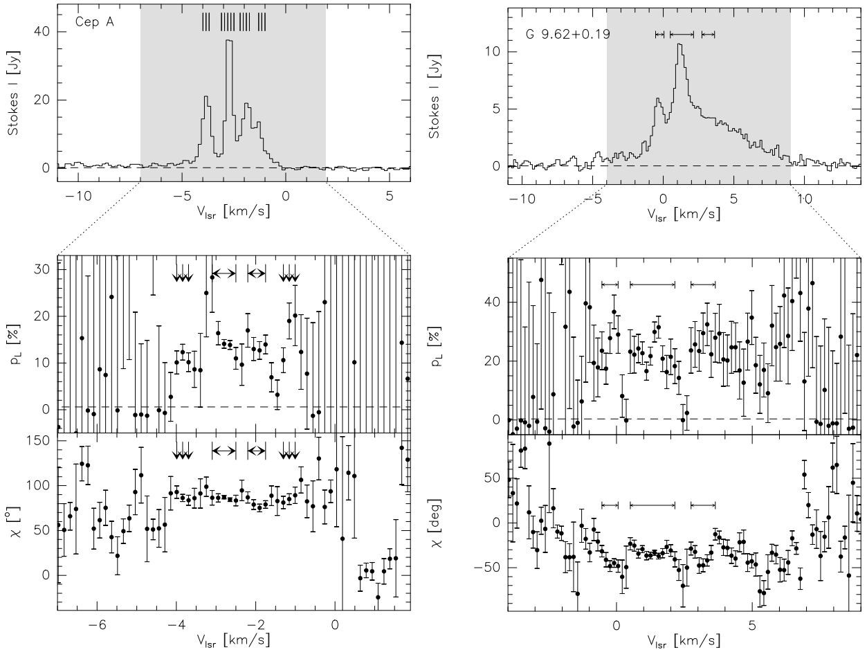
Fig. 6. Class II methanol masers at 157.0 GHz.
