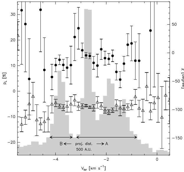
Fig. 11. Overlay of the linear polarization (filled circles, left ordinate) and the polarization angle (unfilled triangles, right ordinate) with the spectrum (grey-shaded) of the 157 GHz CH 3 OH maser towards Cep A. The projected distance of the components A and B is indicated (derived by Mehringer et al. (1997)).
