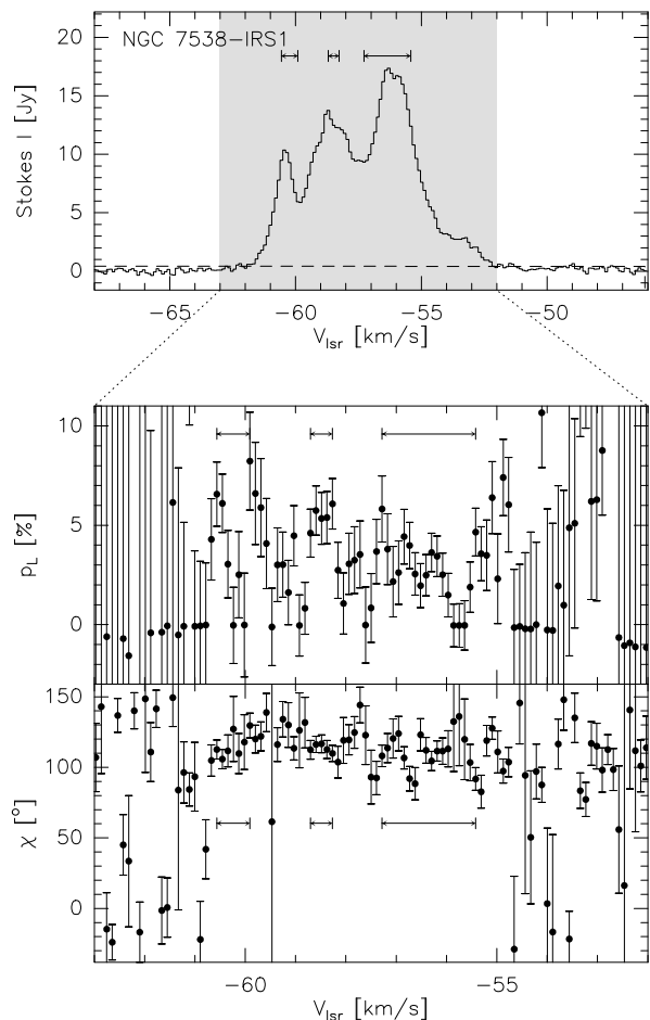
Fig. 5. The 107 GHz polarization spectra of NGC 7538-IRS1, a Class II \text{CH}_3\text{OH} maser.
