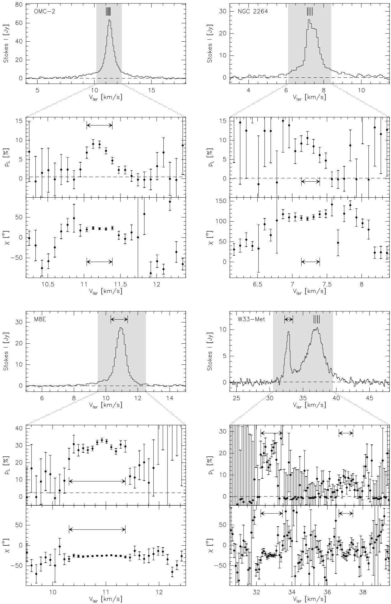
Fig. 4. Class I methanol masers at 132.9 GHz.
