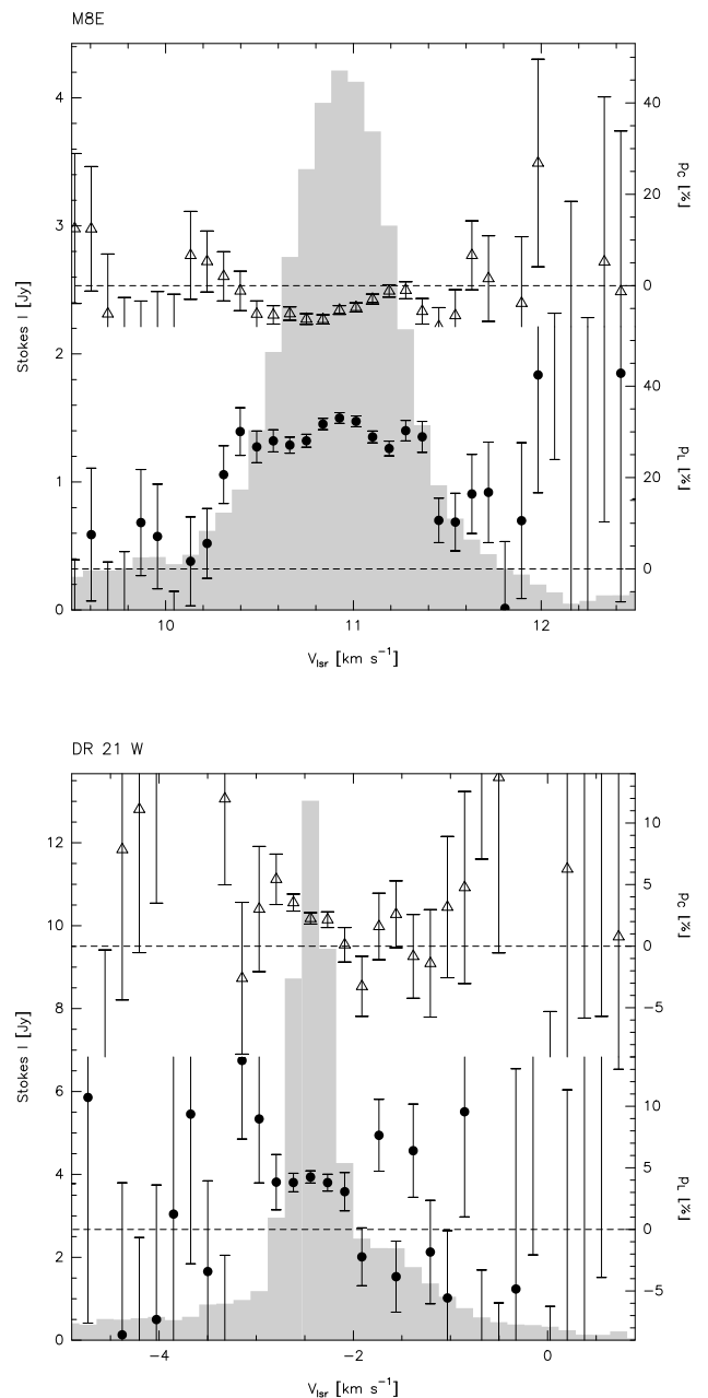
Fig. 10. Detections of circular polarization towards M8E (upper) and DR 21-W (lower), both in the 133 GHz \text{CH}_3\text{OH} maser. The circular polarization p_C is indicated by open triangles, and the linear polarization p_L by filled dots (both on the same scale). The dashed lines indicate the level of zero polarization. For comparison, the Stokes I spectra are shown as grey-shaded histograms. The axes of M8E and DR 21-W are not on the same scale.
