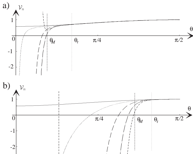
Figure 4: Plot of the five first approximate values \mathcal{V}_n = V + \sum_{p=1}^n (\beta/\varepsilon_n)^{2n} of the soliton velocity \mathcal{V} , against the angle \theta between the propagation direction and the exterior field. The rescaled magnetic induction is m = 1 , and the parameter determining the strength of the exterior field is \alpha = 0.5 . Solid line: n = 0 , dotted line: n = 1 , large dashed: n = 2 , dashed-dotted line: n = 3 , short dashed: n = 4 . For a soliton parameter \beta = 0.1 (a), \beta = 1.5 (b).
