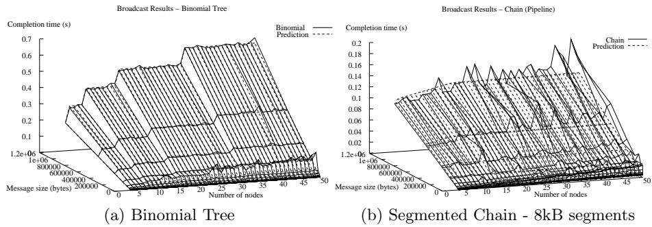
Figure1. Comparison between models and real results
