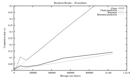
Figure2. Comparison between Chain and Binomial Broadcast
